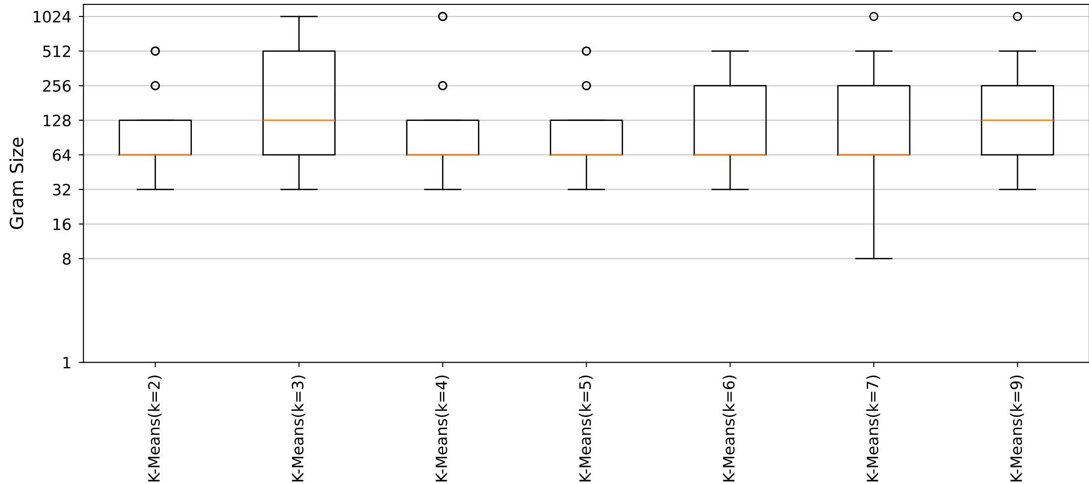
YARA Rules Gram Size Distribution (Cluster12_Size9 dataset)
